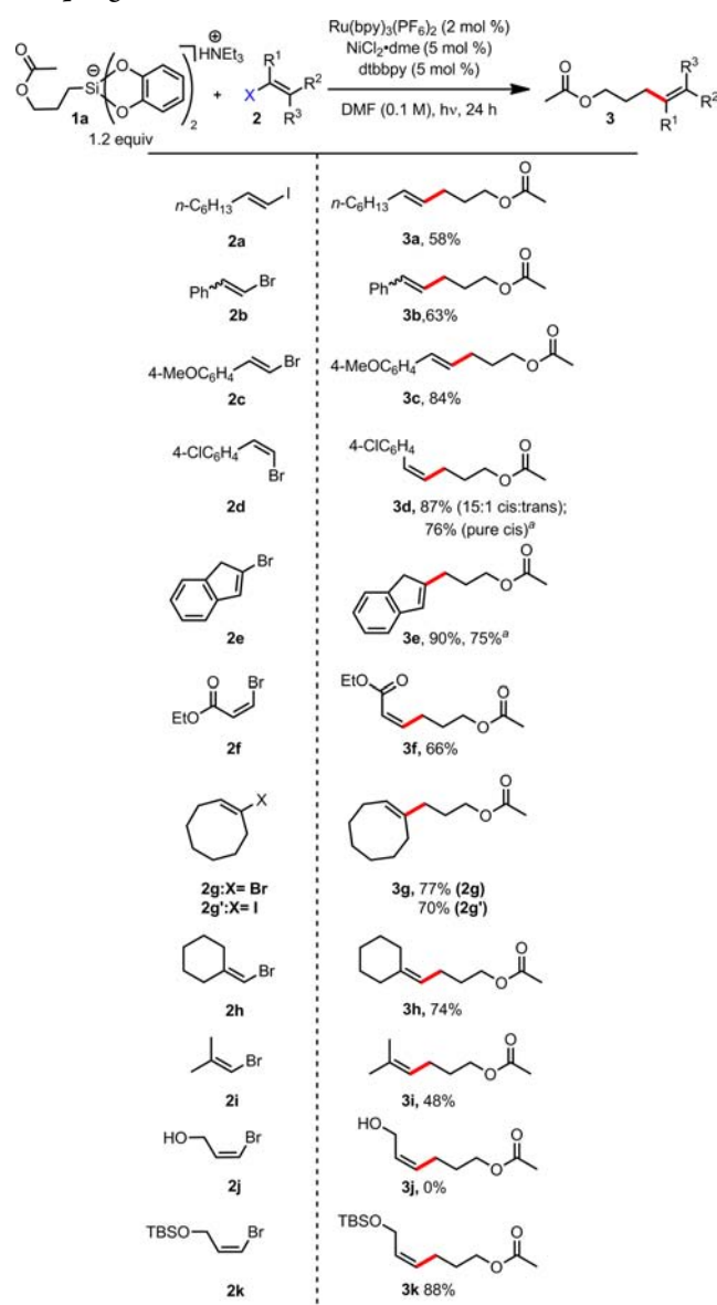
Scheme 3. Scope of Alkenyl Halides in Ni/Photoredox Cross-Coupling
